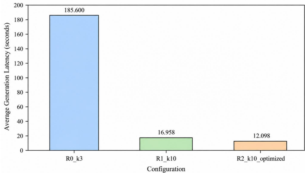
Figure 4: Average Generation Latency Across RAG Configurations
