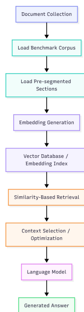
Figure 1: Overview of RAG-Based Document Question-Answering Workflow
